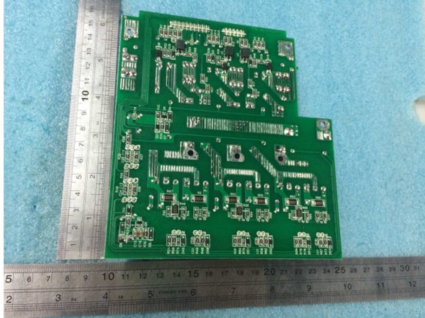
PV side EMI board solder side view:
