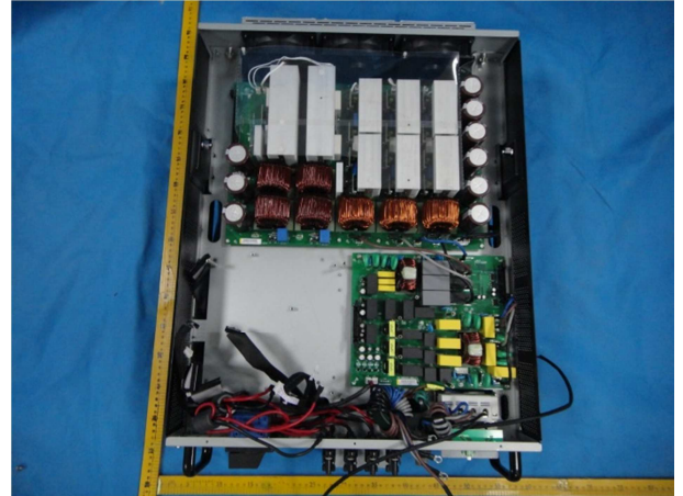
Grid board component side view:
