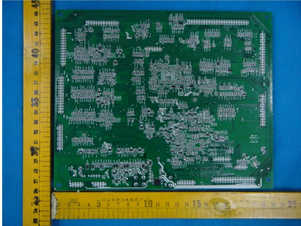
COM board solder side view:
