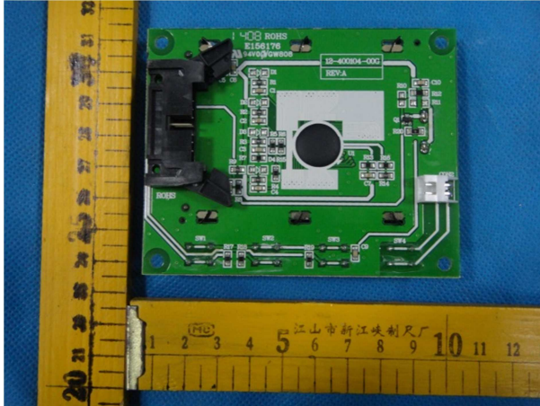
LCD board solder side view:
