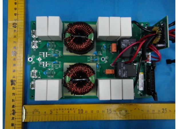
SPS board component side view:
