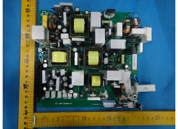
Relay board component side view:
