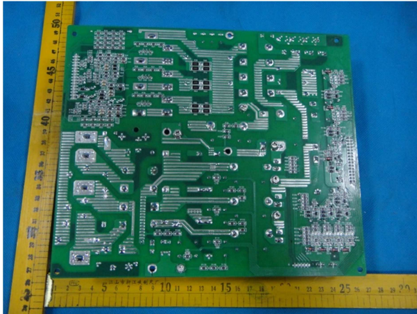
Inverter board solder side view:
