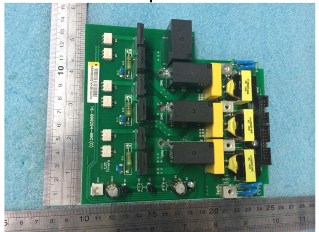
OP board component side view:
